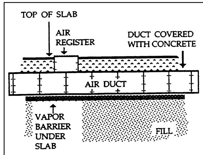
Figure 6-8. Subslab air duct system.
