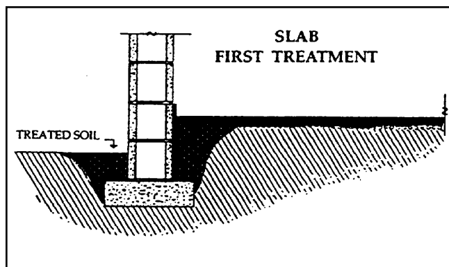
Figure 6-1. Termiticide treatment of the fill material prior to pouring a concrete slab protects wood in the building from termite attack.
