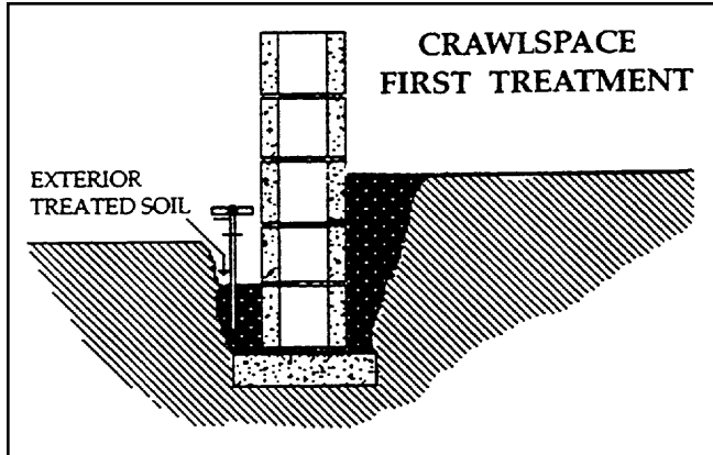
Figure 6-3. Preconstruction treatment of inside and outside foundation perimeter.
