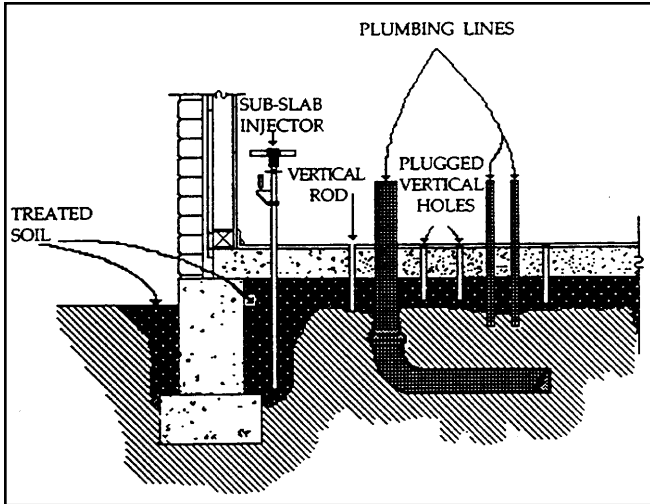
Figure 6-5. Treatment under concrete slab with vertical rodding at joints, cracks, and openings around plumbing.
