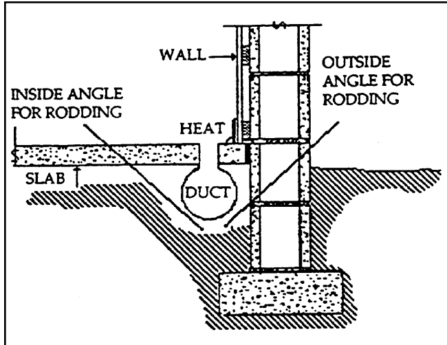
Figure 6-9. Subslab perimeter heat duct showing the angles needed to rod the termiticide system.
