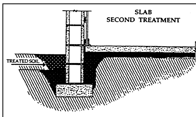
Figure 6-2. Application of a termiticide to soil around the foundation.
