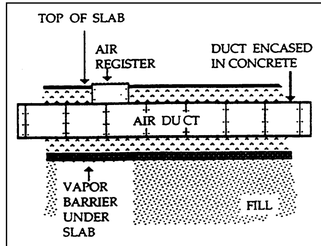
Figure 6-7. Intraslab air duct system.
