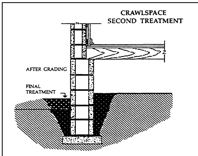
Figure 6-4. Second treatment after the final grading.
