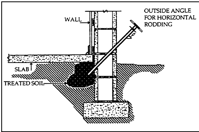
Figure 6-6. Horizontal rodding through exterior wall.
