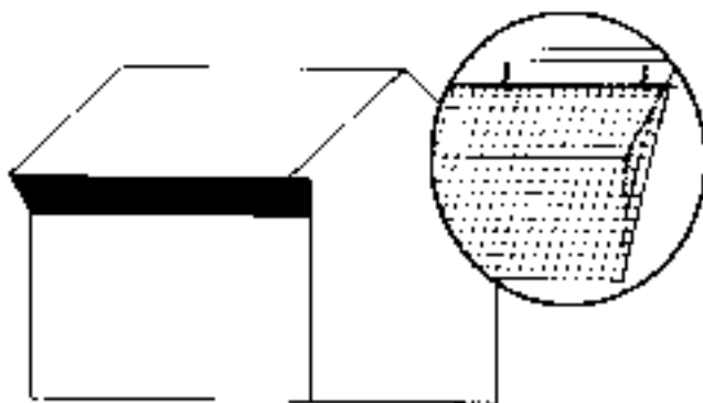
Figure 2. Netting mounted on building from the outside edge of the eave down to the side of the building. Insert shows a method of attachment using hooks and dowels.
